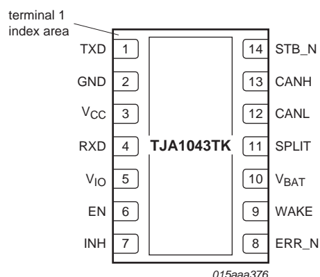
Fig 3. Pin configuration diagram: HVSON14
