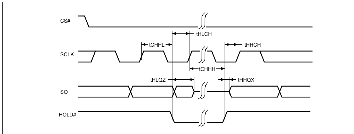
Figure 9. Hold Timing
