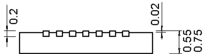
QFN28_4X4
