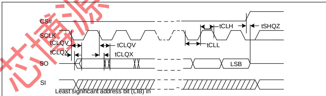
Figure 39. Output Timing
