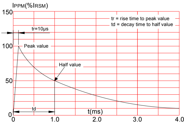
FIG.2: Pulse waveform
