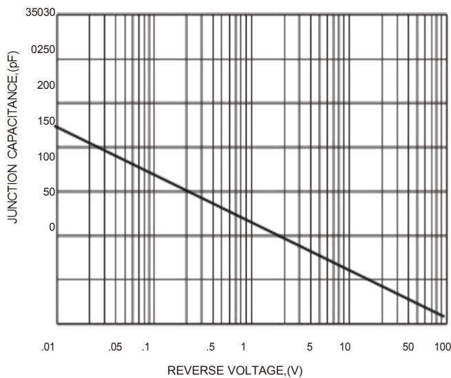
FIG.4-TYPICAL JUNCTION CAPACITANCE
