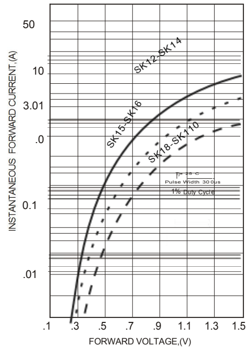
FIG.2-TYPICAL FORWARD CHARACTERISTICS
