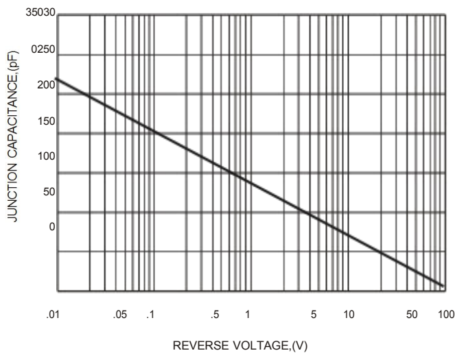
FIG.4-TYPICAL JUNCTION CAPACITANCE
