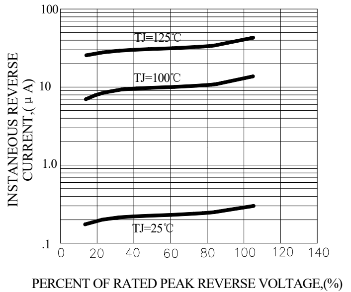
FIG.4-TYPICAL REVERSE CHARACTERISTICS
