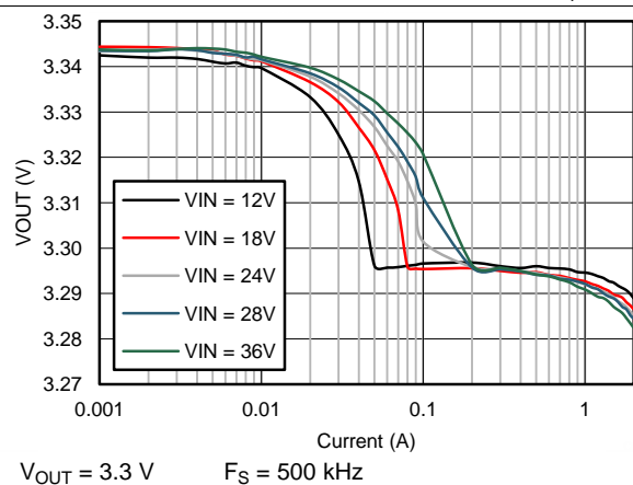
Figure 7. V_{OUT} Regulation
