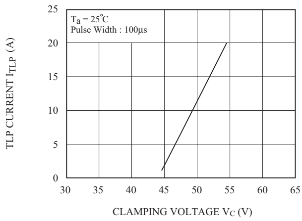
TLP CURVE
